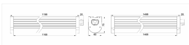
Product Dimension
