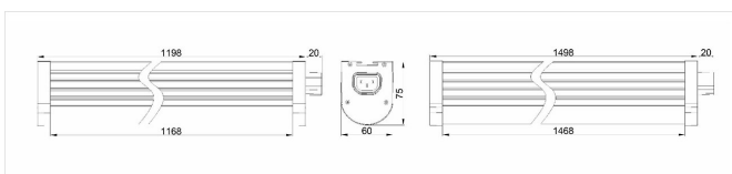
Product Dimension
